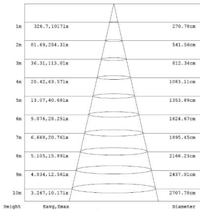
Diagram for R300LEDC40N-01 in 4000K. Other diagrams available on request
