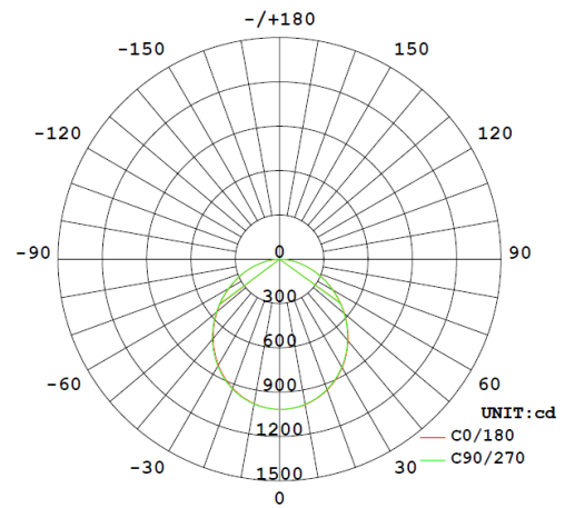
Diagram for R300LEDC40N-01 in 4000K. Other diagrams available on request
